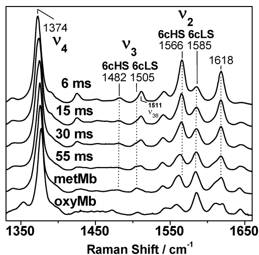
Figure 2. High-frequency RR spectra obtained with 413-nm excitation at 105 K on RFQ samples (reaction times: 6, 15, 30, and 55 ms) of Mb–O 2 + NO at pH 9.5. Also shown are the RR spectra of the product and starting material at pH 9.5, metMb and oxyMb, respectively.
