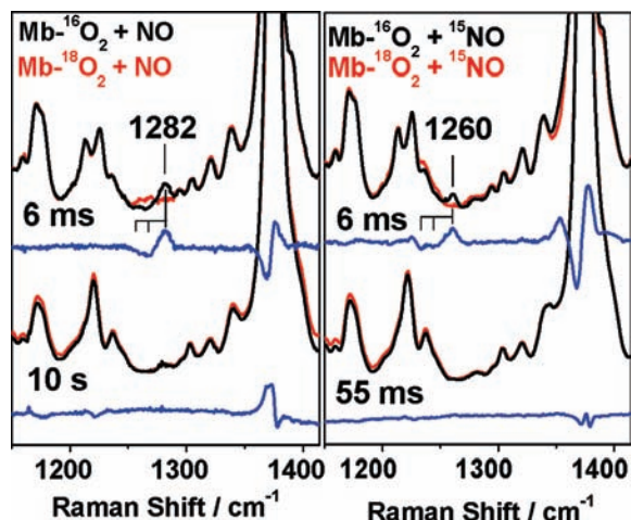
Figure 3. Midfrequency RR spectra of RFQ samples for the reaction of ^{14}\text{NO} (left) and ^{15}\text{NO} (right) with \text{Mb-}^{16}\text{O}_2 (black) versus \text{Mb-}^{18}\text{O}_2 (red). Difference spectra are shown in blue; the differential signals occurring at the intense \nu_4 mode ( 1374\text{ cm}^{-1} ) vary in independent experiments and represent less than 10% of the integrated \nu_4 area.
