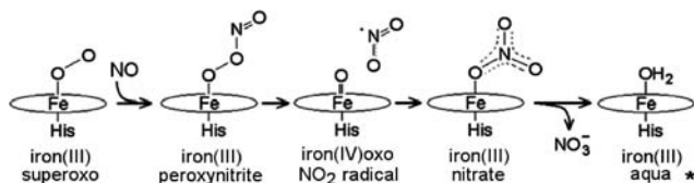
Figure 1. Proposed NO dioxygenation by oxyheme (* at alkaline pH, the iron(III) aqua complex of myoglobin is replaced by an iron(III) hydroxo complex, which adopts a low-spin configuration at cryogenic temperatures).
